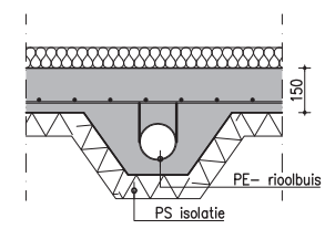
principe detail A-A schaal 1:20
